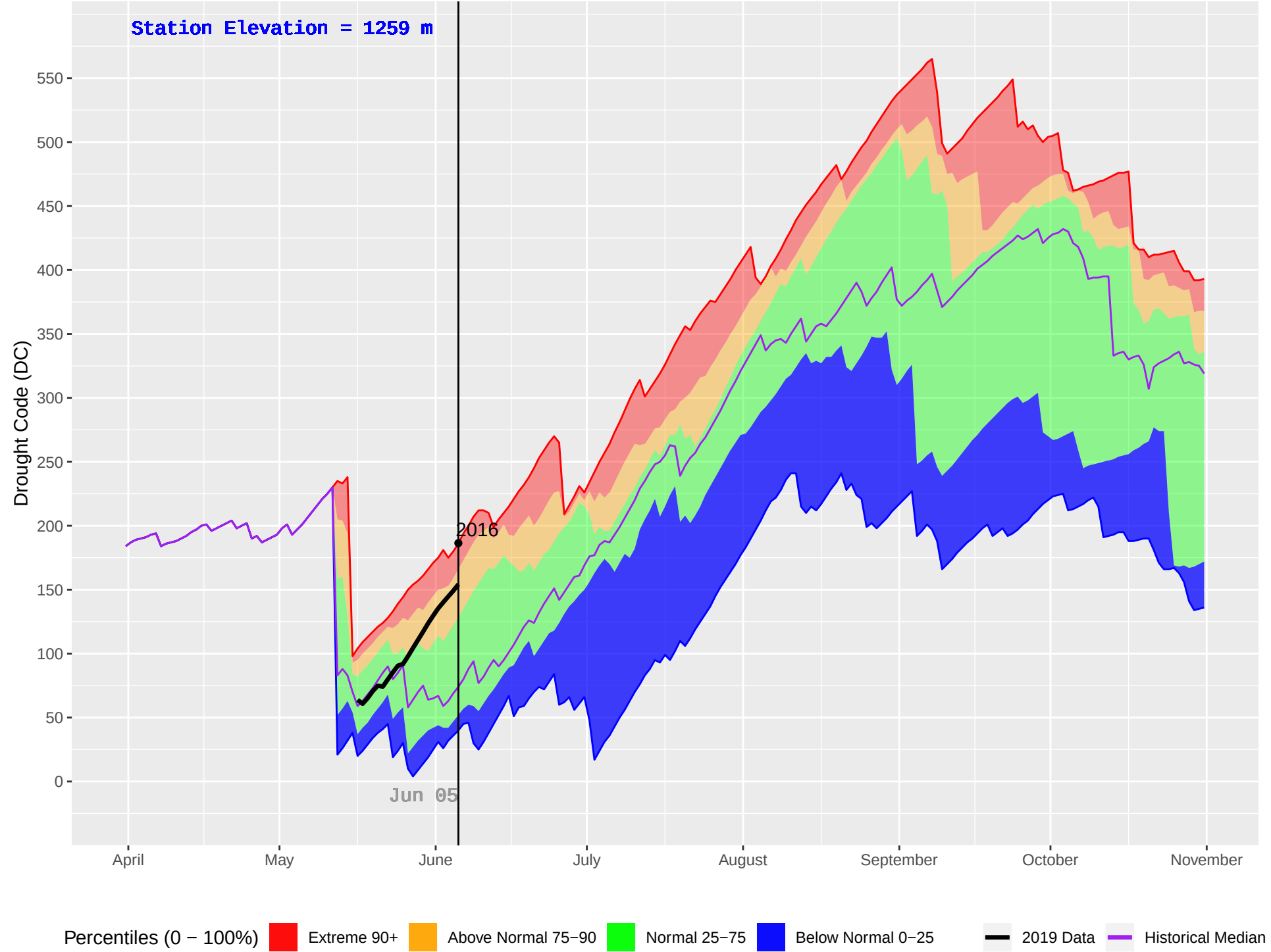
PARROTT (183) : Historical (1995–2018) and Current (2019) Daily Drought Code (DC)
