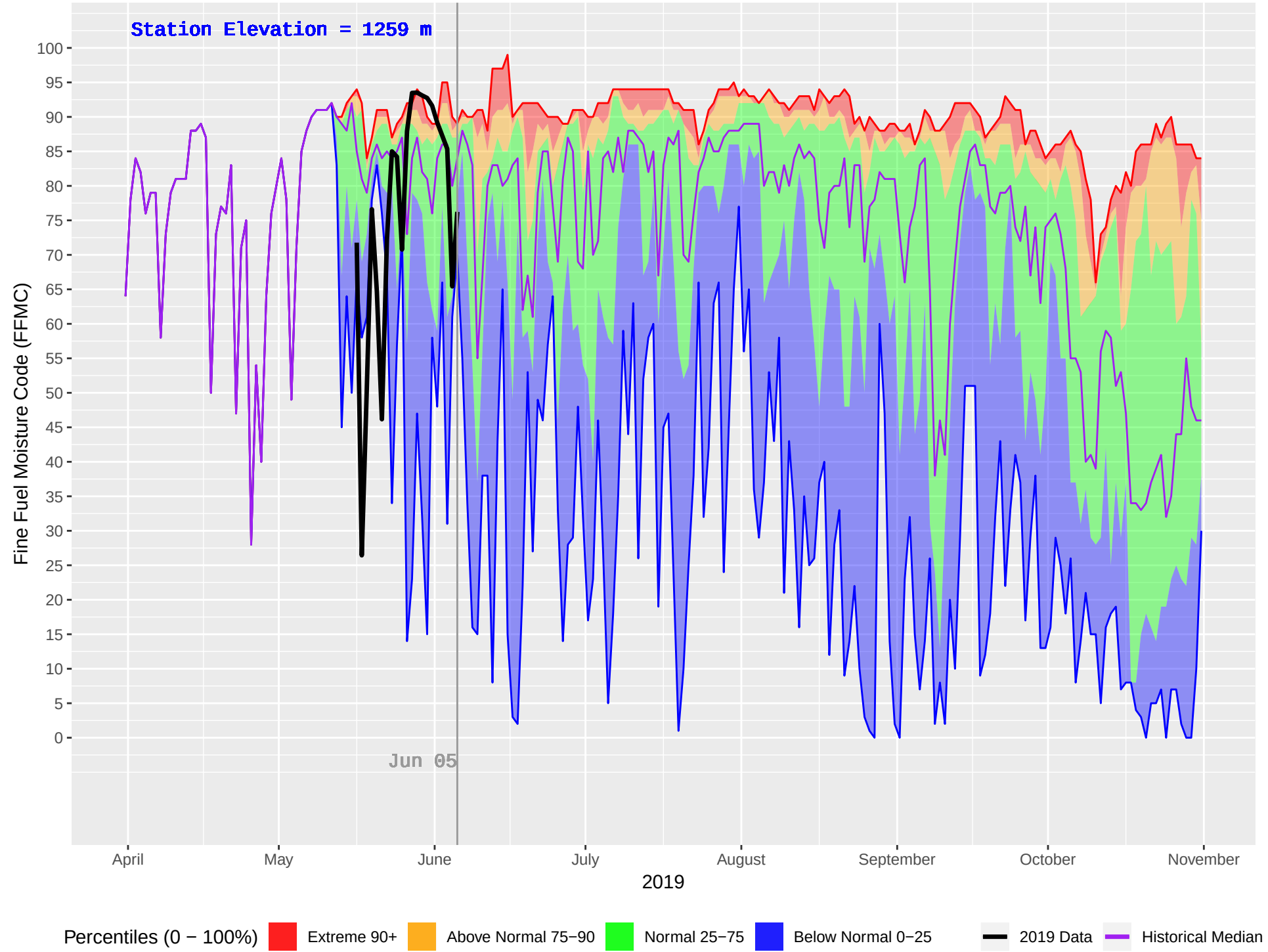
PARROTT (183) : Historical (1995–2018) and Current (2019) Daily Fine Fuel Moisture Code (FFMC)
