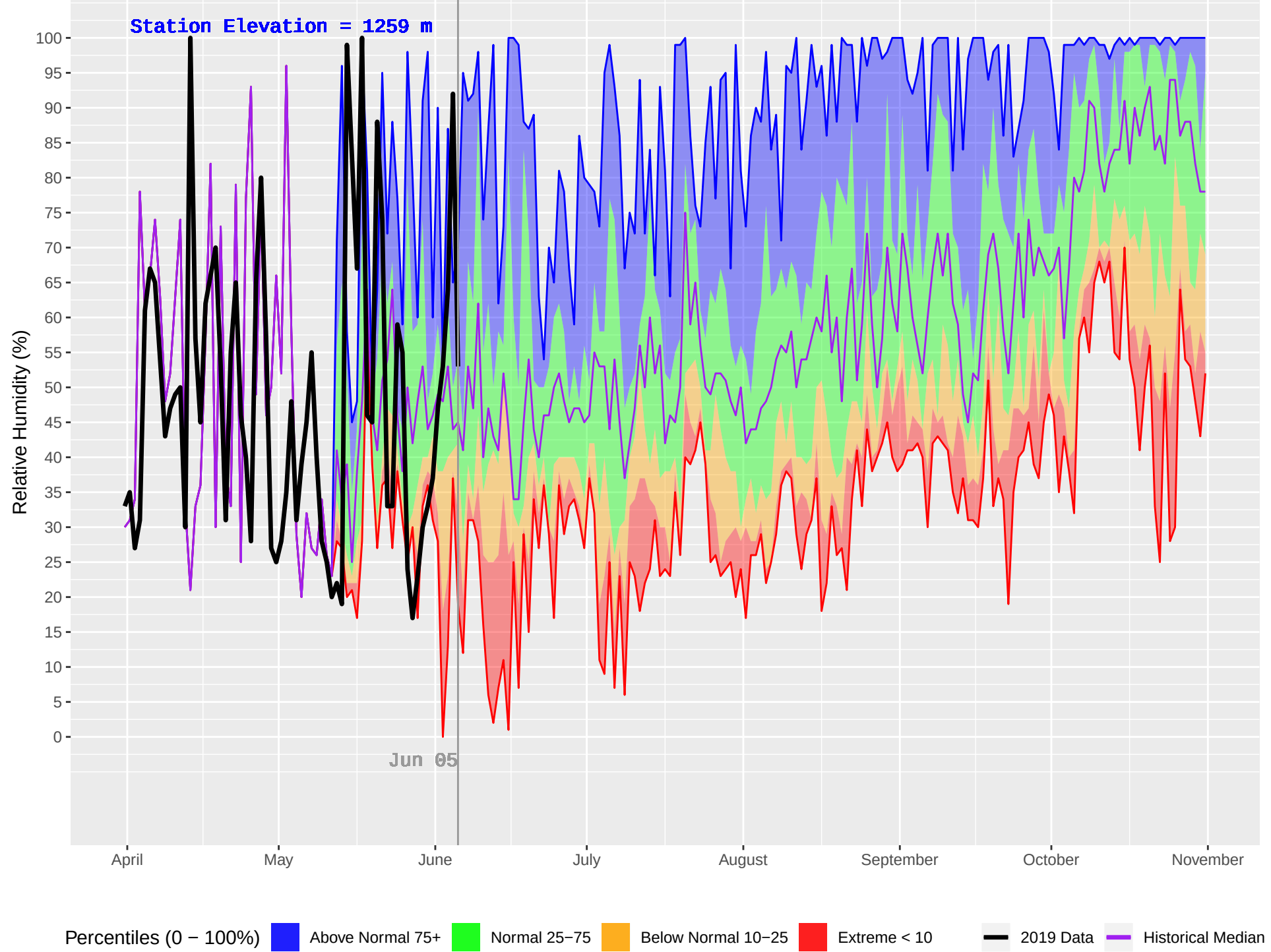
PARROTT (183) : Historical (1995–2018) and Current (2019) Daily Relative Humidity
