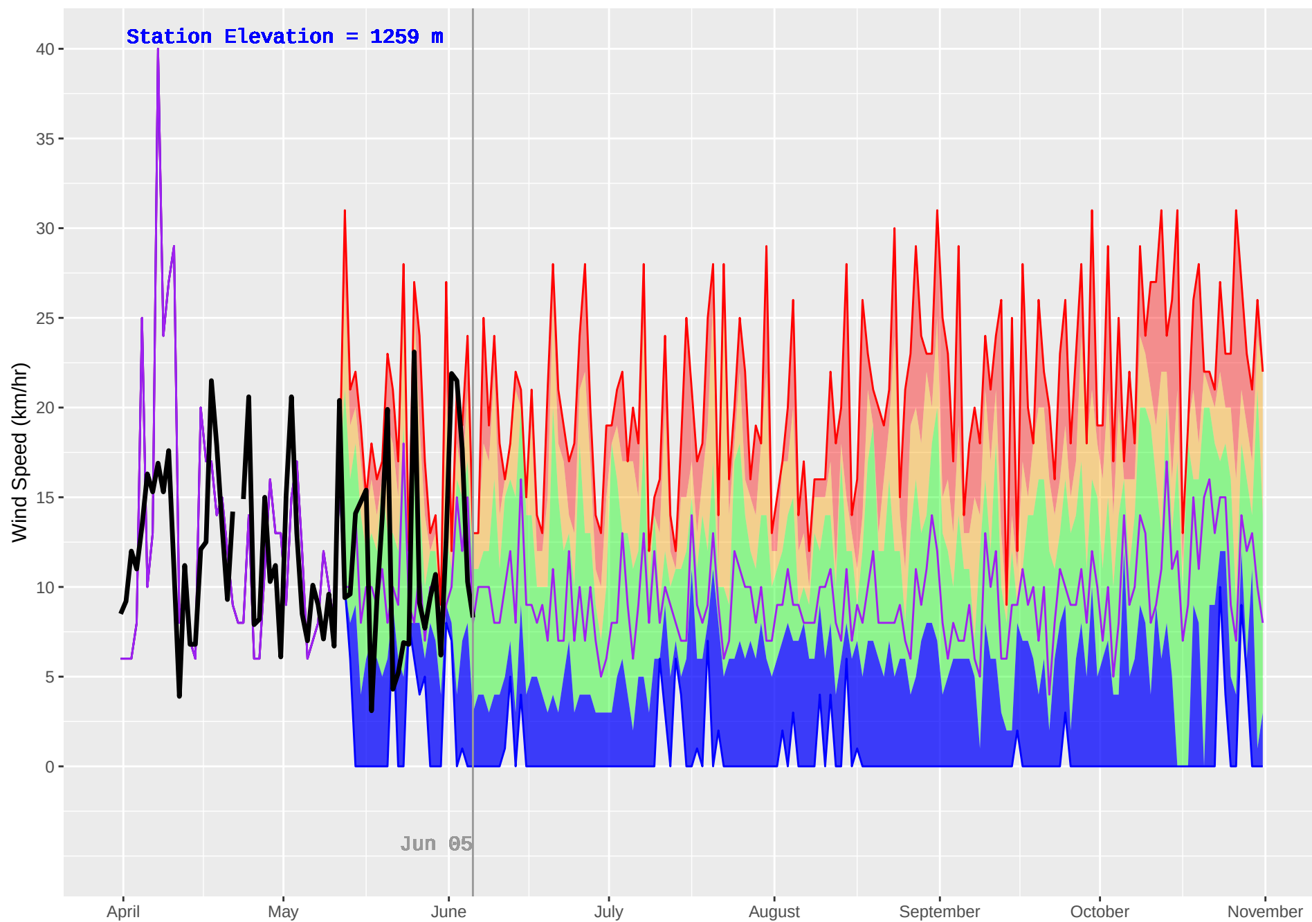
PARROTT (183) : Historical (1995–2018) and Current (2019) Daily Wind Speed
