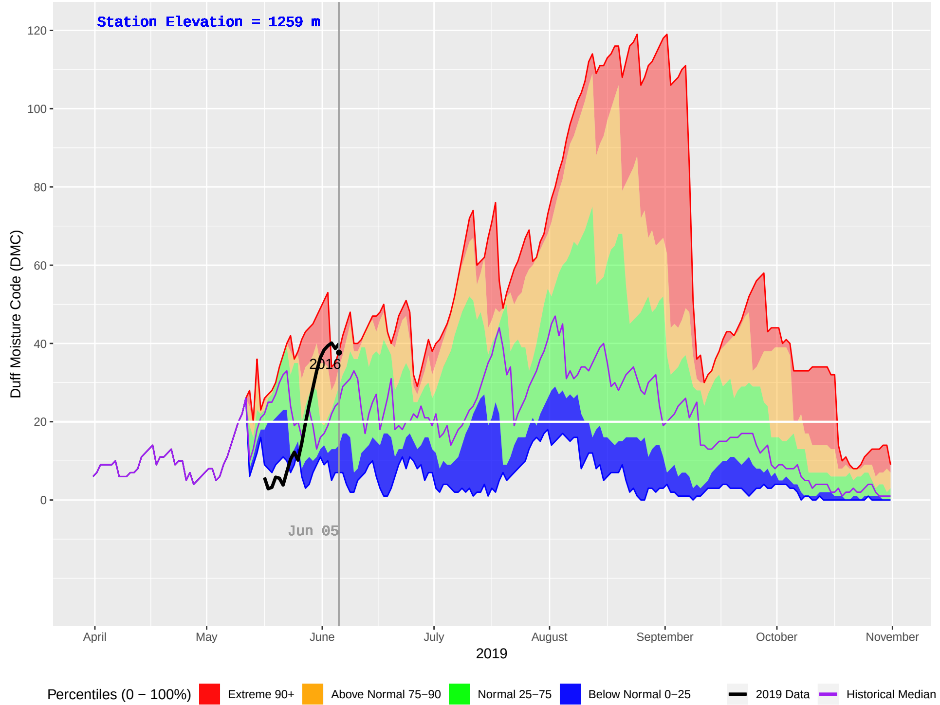
PARROTT (183) : Historical (1995–2018), Current (2019) Daily Duff Moisture Code (DMC)
