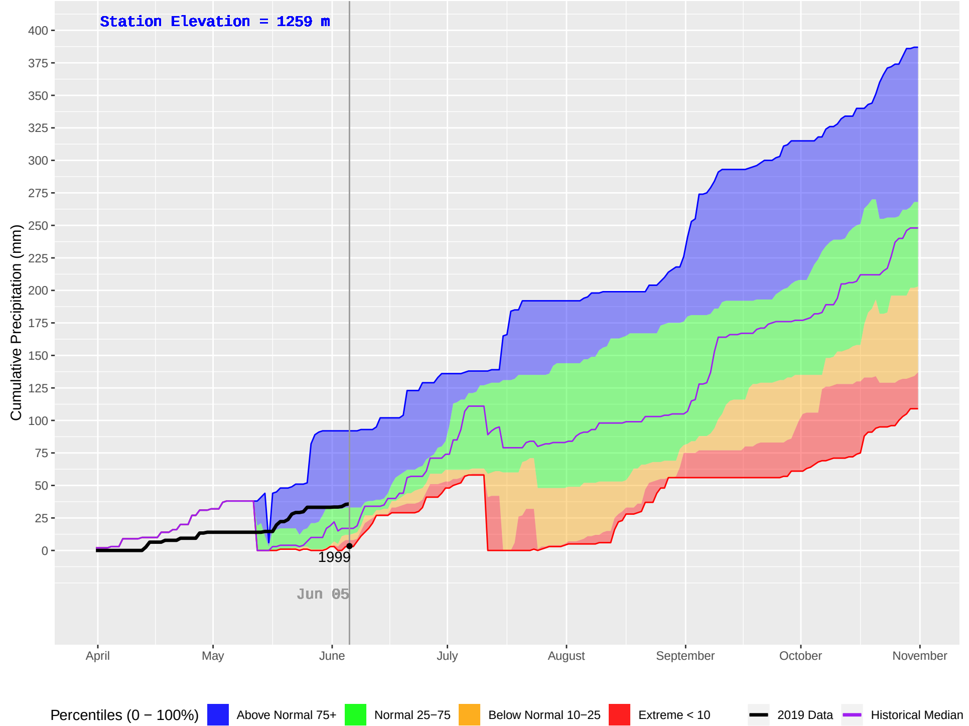
PARROTT (183) : Historical (1995–2018), Current (2019) Daily Cumulative Precipitation
