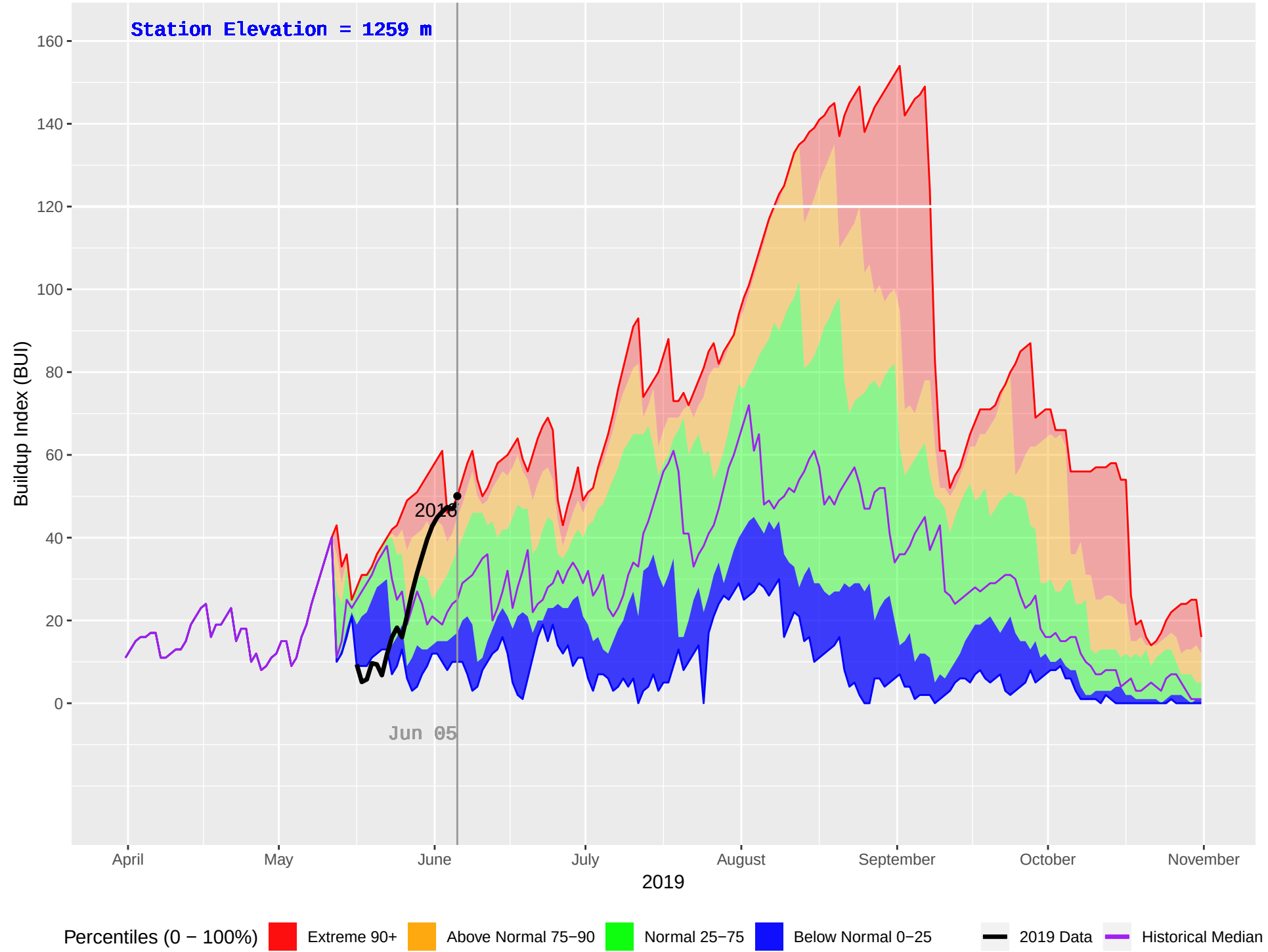
PARROTT (183) : Historical (1995–2018), Current (2019) Daily Buildup Index (BUI)
